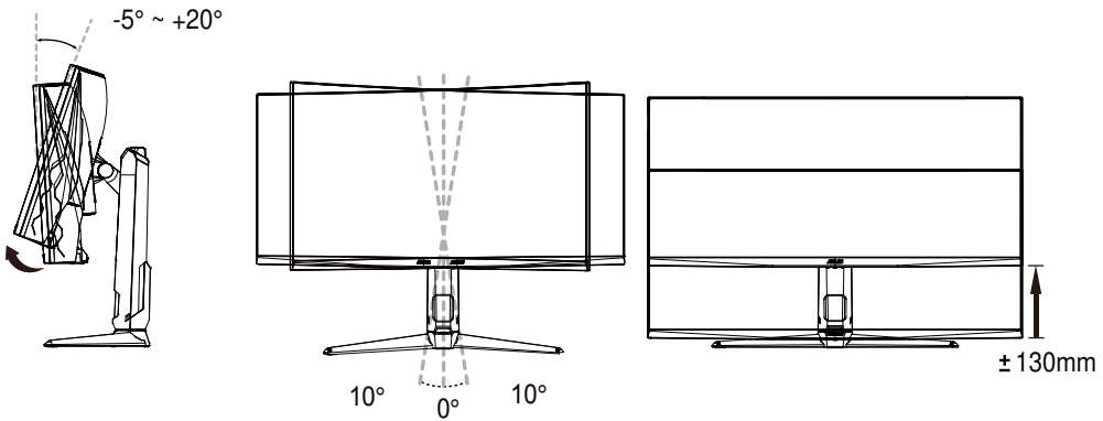
(Height adjustment)
